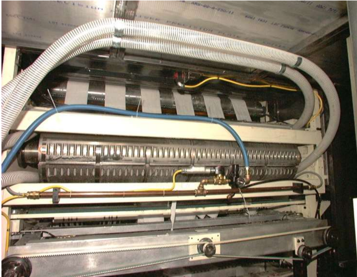
078-Inside_Folder_Guarding
